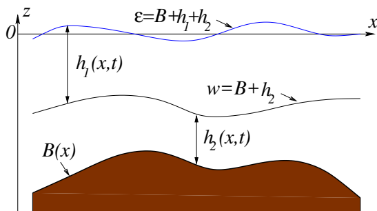
Figure 7.1. Set-up for the two-layer shallow-water system (7.6).
